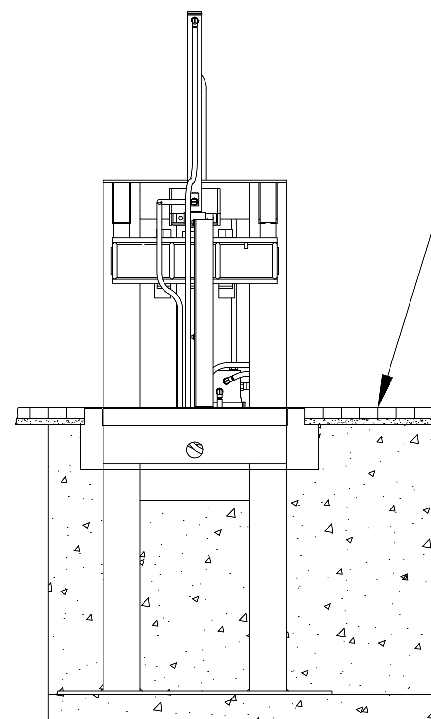
SIDE (ELEVATION) VIEW
